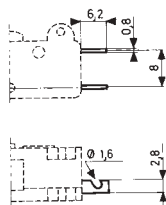
W2 Solder End Terminals
