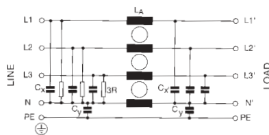
PFT-25B/36B/50B/65B/80B/110B/150B Series Circuit Schematic
