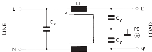
PE Series Circuit Schematic
