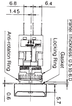
Rectangular Push-button
